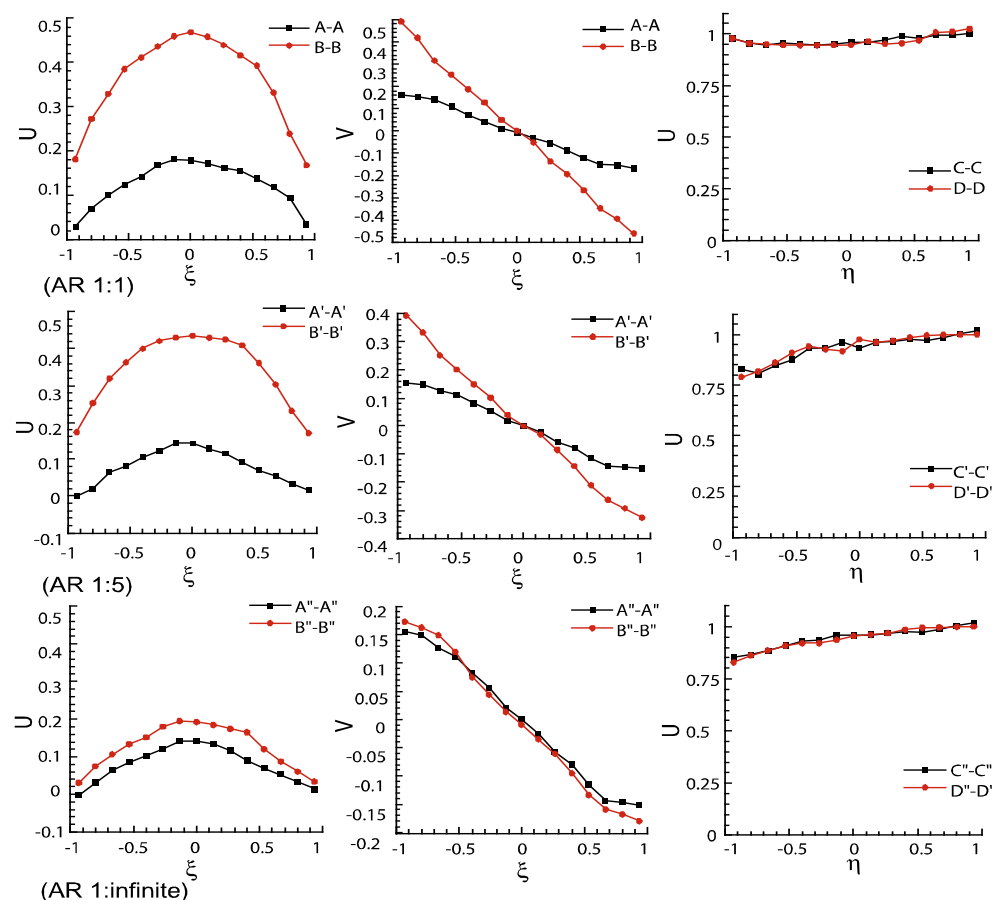
Fig. 5. Point-wise comparisons of the stream-wise velocity, U , and cross-stream velocity, V , in the T-junctioned channels (AR 1:1, AR 1:5, and AR 1:infinite) at each section.
