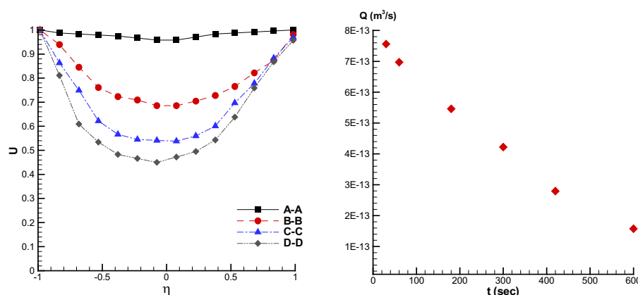
Fig. 3. Point-wise comparisons of the stream-wise ( U ) velocity at A-A, B-B, C-C and D-D sections (left) and volume flow-rate vs. time in the straight microchannel (right).
