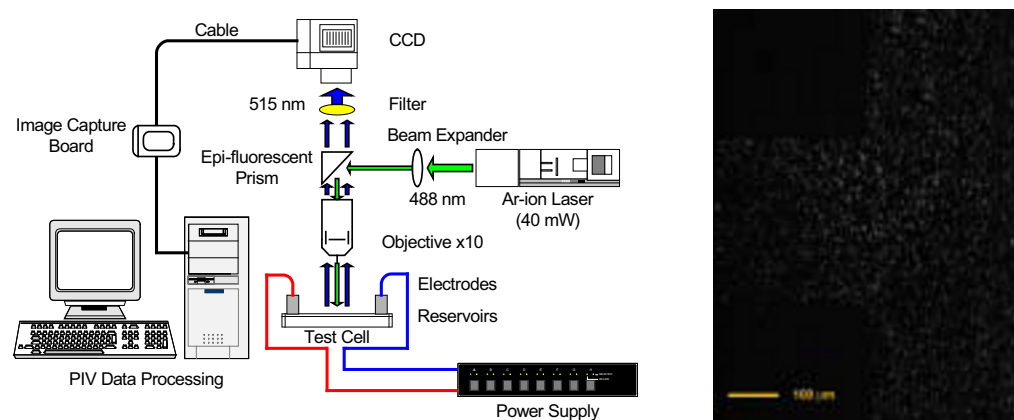
Fig. 1. Experimental setup for microscopic PIV system and PIV image in the T-junctioned microchannel.
