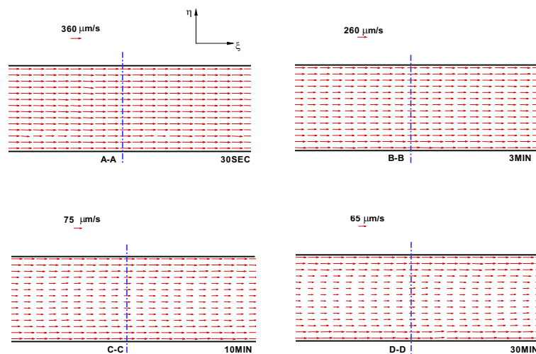
Fig. 2. Time development of the global velocity distribution for electro-osmotic flow.
